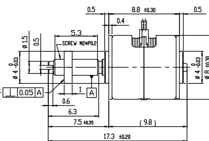
21SRL0808001 STEPPING MOTOR
