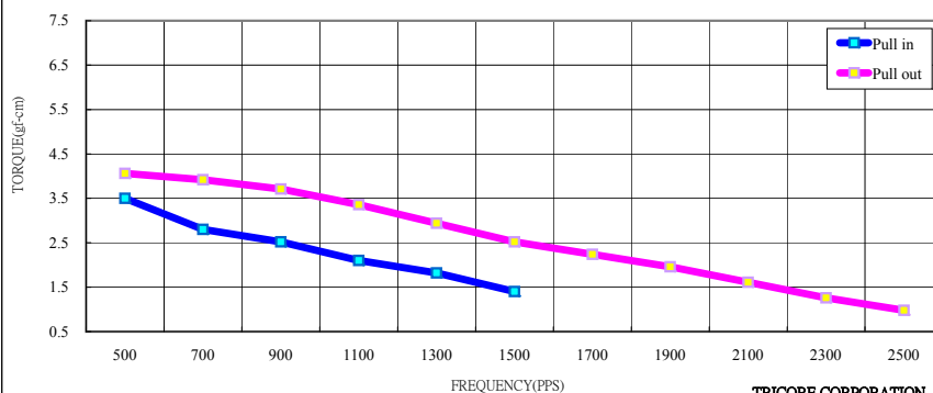
21SRL0808001 STEPPING MOTOR
