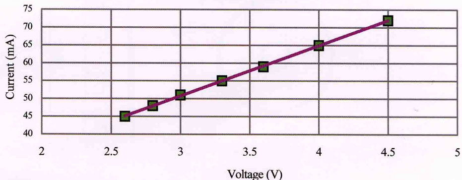
Φ10 Vibration Motor V-A Curve
